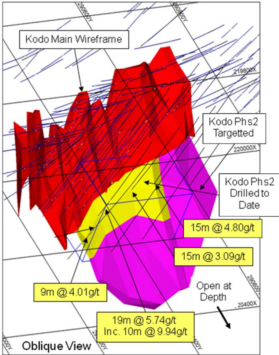
Figure 1. Oblique view of the Kodo resource, and newly drilled area (100m x 100m grid shown)
