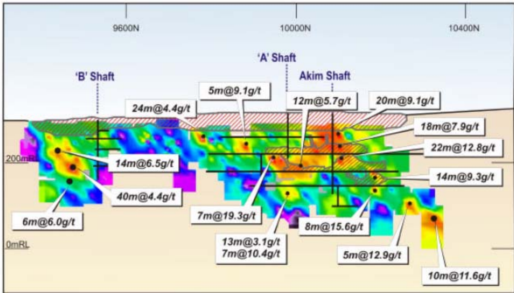
Longitudinal section of Obenemase deposit showing NE plunging shoots
