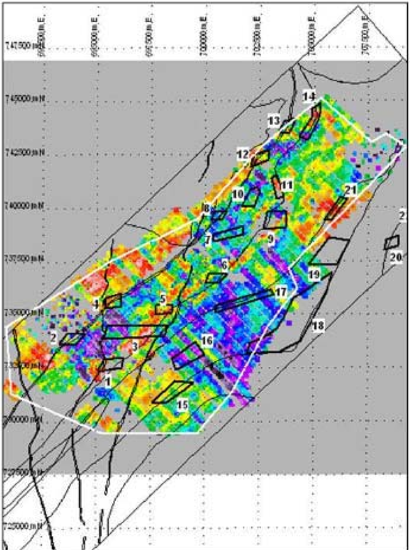
Structural target areas on Ar geochemistry
