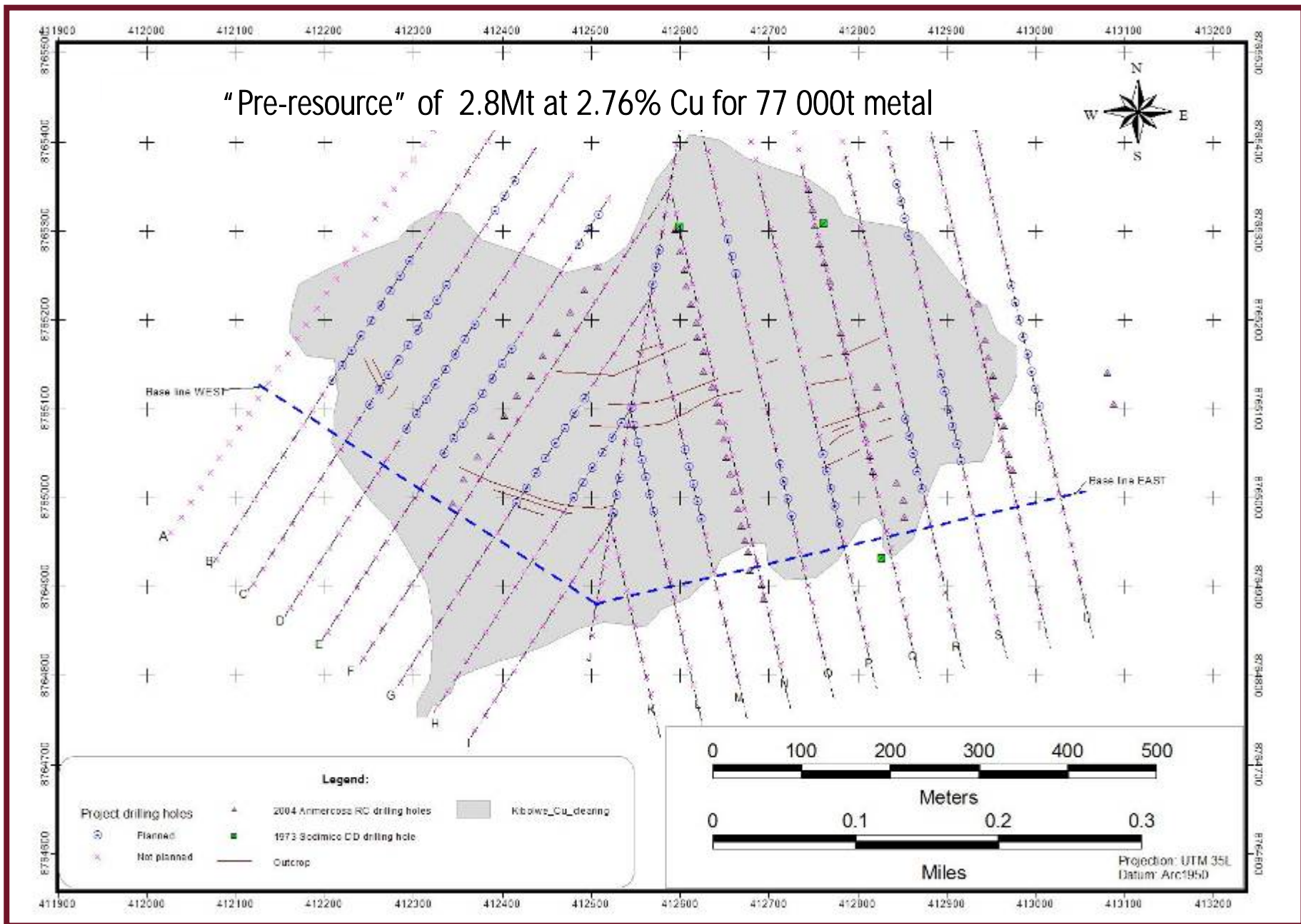
Kibolwe Cu clearing drill plan
