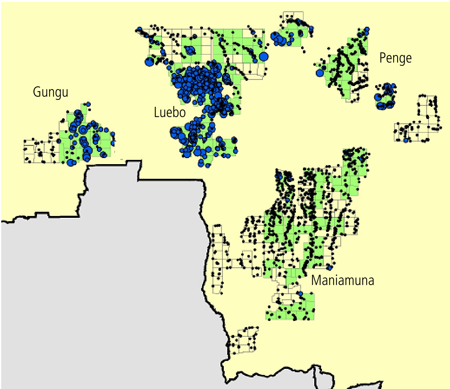
Gravity exploration areas showing total ilmenite counts
